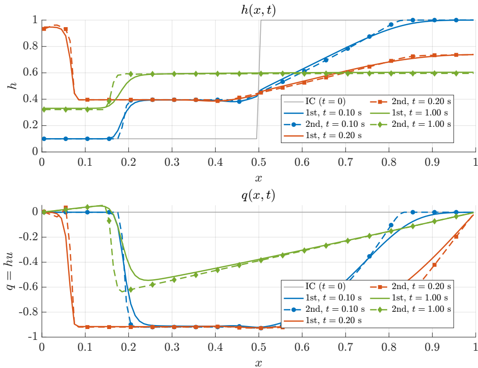
Case (b): Reverse Dam Break — \Delta x = 0.0100 , CFL = 0.20, \Delta t_{\text{avg}} \approx 0.5316 ms
