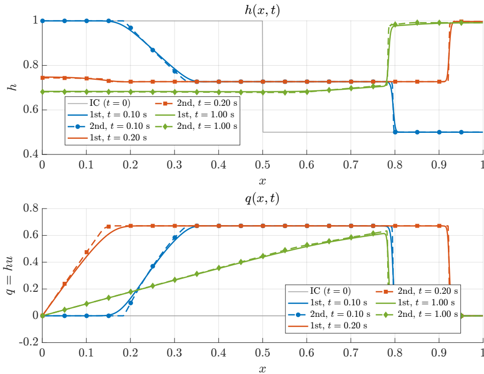
Case (c): Hydraulic Jump — \Delta x = 0.0013 , CFL = 0.15, \Delta t_{\text{avg}} \approx 0.0531 ms
