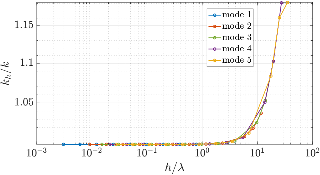
Dispersion curve
