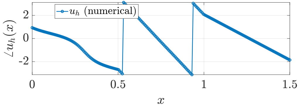
Phase of u_h ( h = 0.0075 , n_{\text{El}} = 200 )
