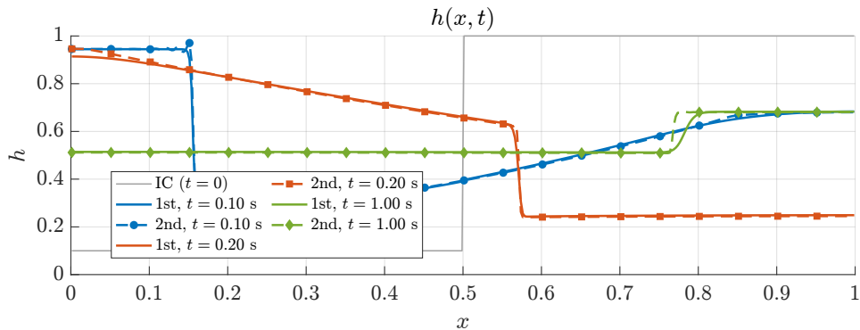
Case (b): Reverse Dam Break, h_{ref} = 0.05 , \Delta x = 0.0025 , CFL = 0.20, \Delta t_{avg} \approx 0.0580 ms
