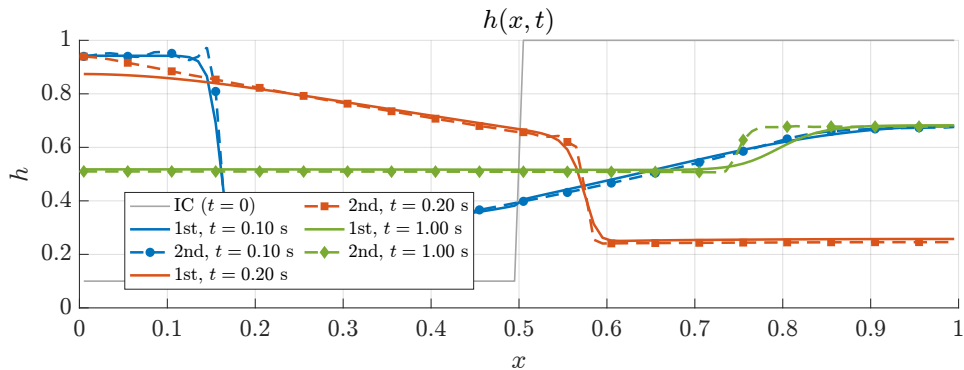
Case (b): Reverse Dam Break, h_{ref} = 0.05 , \Delta x = 0.0100 , CFL = 0.20, \Delta t_{avg} \approx 0.2370 ms
