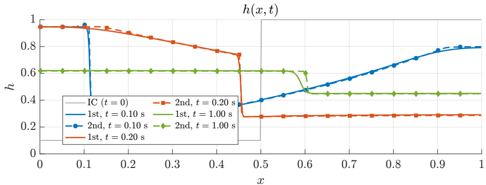
Case (b): Reverse Dam Break, h_{ref} = 0.10 , \Delta x = 0.0025 , CFL = 0.20, \Delta t_{avg} \approx 0.0644 ms
