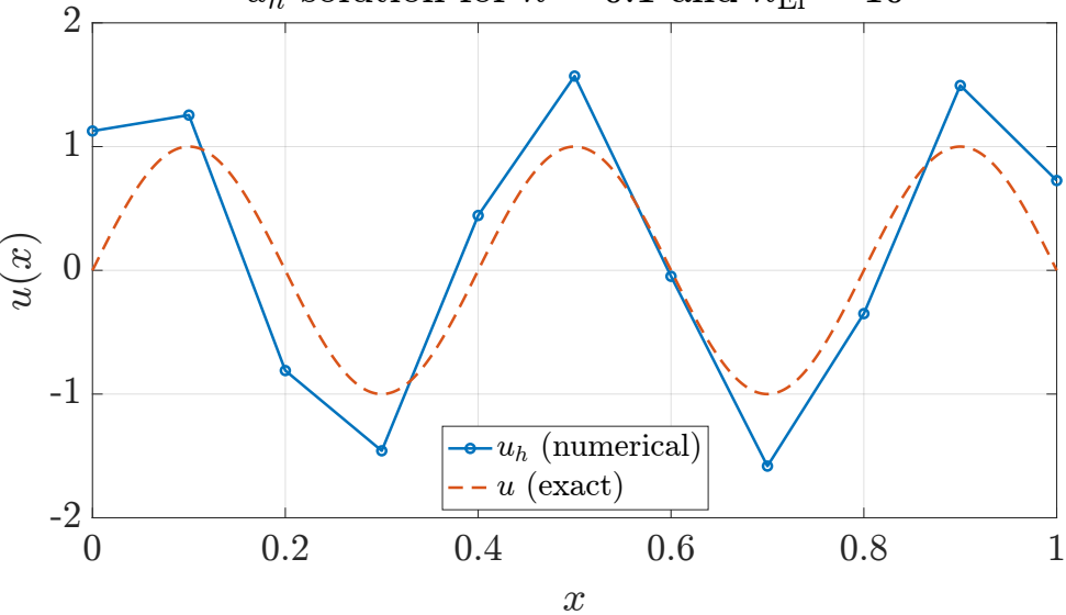
u_h solution for h = 0.1 and n_{\text{El}} = 10
