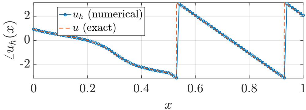
Phase of u_h ( h = 0.01 , n_{\text{El}} = 100 )
