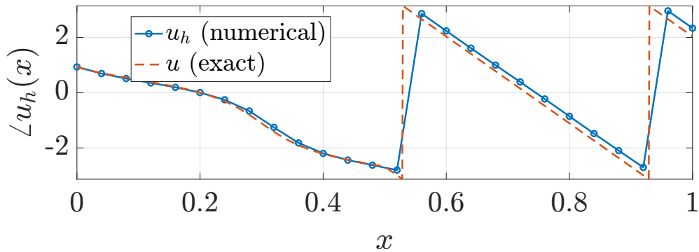
Phase of u_h ( h = 0.04 , n_{\text{El}} = 25 )
