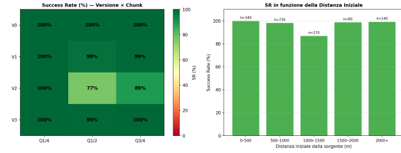
Figura 6: Success rate per scenario — minimal.
