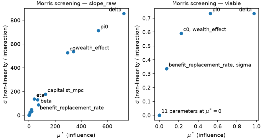
Figure 9: Morris screening of seventeen parameters—the sixteen defensible parameters plus max_tax , which is screened here only. In the viability panel eleven parameters share \mu^* = 0 —no measurable effect on viability—and are drawn as one labelled cluster rather than eleven overlapping points: beta , c1 , capitalist_mpc , eta , expectation_gain , investment_floor , max_tax , pct_capitalists , target_utilization , u_min , wage_floor . Parameters sharing a coordinate are labelled jointly, and singletons whose \mu^* is at or below 5% of the panel maximum are left unlabelled. The chord estimator ( ces_b13 ).
