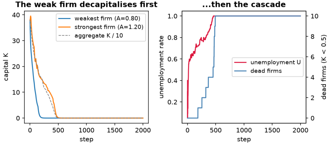
Figure 6: The domino behind the cliff (headline scenario c_0 = 1.0 , \sigma = 0.5 , \eta = 0.10 ; productivity spread 0.20; seed 0). Left: the weakest firm decapitalises first, then the strongest. Right: unemployment climbs as firms die, through the demand externality—laid-off workers lose their income—and the spending shares left pointing at the dead firm.
