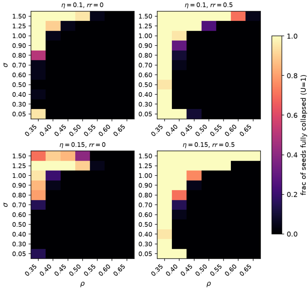
Figure 8: The other face: the demand floor enlarges the collapse region ( c_0 = 2.0 ). The map uses categorical axes—one cell per simulated node, all cells the same width—because the \sigma grid is non-uniform (nodes at 0.05, 0.30, 0.40, \dots , 1.25, 1.50); ticks fall only on simulated nodes, so no colour is read off a \sigma the grid does not contain.
