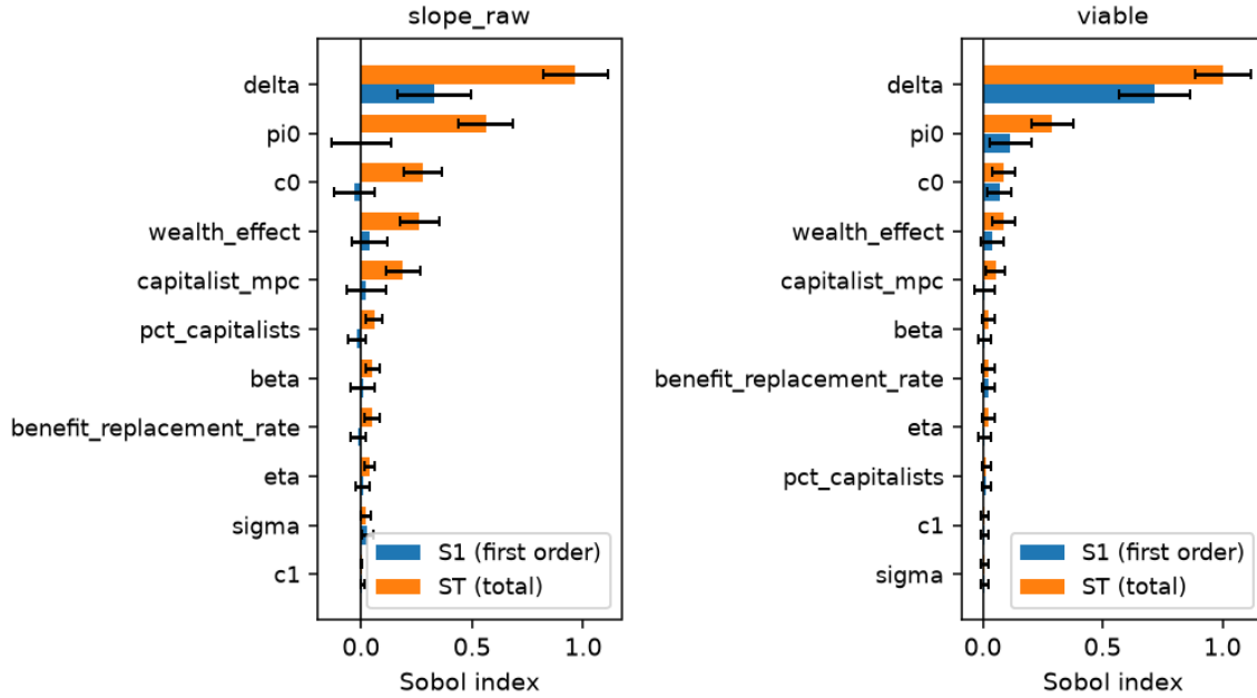
Figure 10: Sobol' indices with bootstrap confidence intervals, over the sixteen-parameter defensible space, on the chord estimator ( ces_b13 ); Fig. 11 is the OLS-repaired counterpart ( ces_b14 ).
