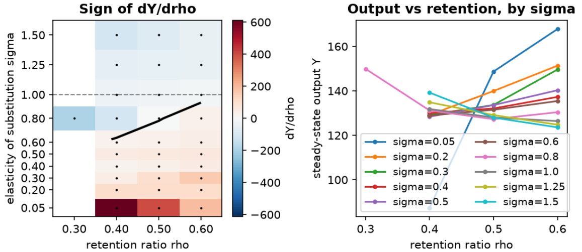
Figure 3: Sign of dY/d\rho over the (\sigma, \rho) grid. In the map (left) blue is the wage-led region ( dY/d\rho < 0 , retention lowers output) and red the profit-led region; the black curve is the zero contour—the sign frontier itself. The \sigma grid is non-uniform (nodes at 0.05, 0.20, 0.30, \dots , 1.25, 1.50; \rho at 0.30–0.60), so ticks fall only on simulated nodes and a dot marks each of the 31 measured cells; the remaining 9 of 40 are non-viable, carry no derivative, and are left blank. The zero contour is interpolated between nodes, and its position between two \sigma rows is read as such. The dashed line marks \sigma = 1 . Steady-state output against retention, one curve per \sigma (right).
