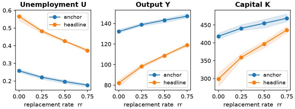
Figure 7: The first face of the balanced-budget benefit: dose-response of steady-state U , Y and K against the replacement rate rr , with inter-seed bands. The benefit lowers unemployment and—the theoretical point—raises capital, crowding investment in within the demand-constrained regime.
