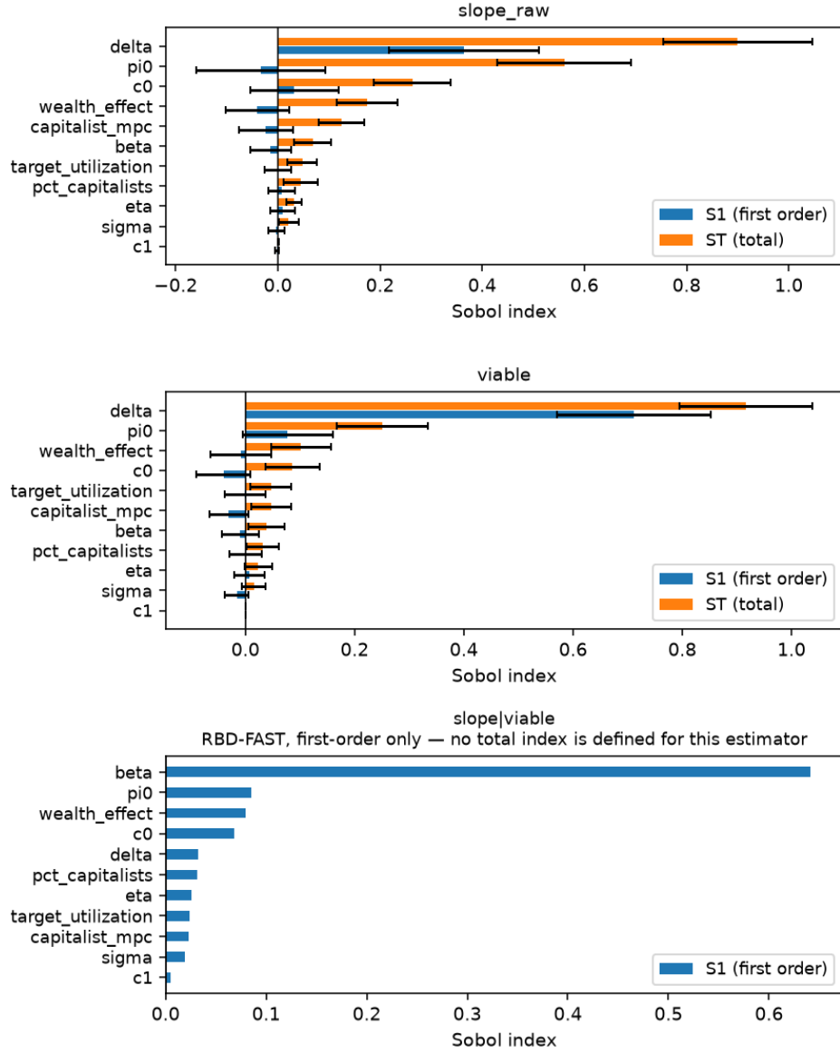
Figure 11: The same decomposition on the OLS-repaired QoI (ces_b14), the counterpart of the chord-based Fig. 10. On the slope the total indices barely move from the chord values reported in Section 9.2: \delta reads 0.900, \pi_0 reads 0.561, and \sigma reads 0.021; on viability \delta reads 0.916. The survivor set differs from Fig. 10 (target_utilization enters, benefit_replacement_rate leaves), so the vertical axis is not identical. The third panel is the conditional quantity slope | viable under RBD-FAST, which defines only a first-order index, no total index is shown, and it is the panel in which the accelerator gain \beta dominates.
