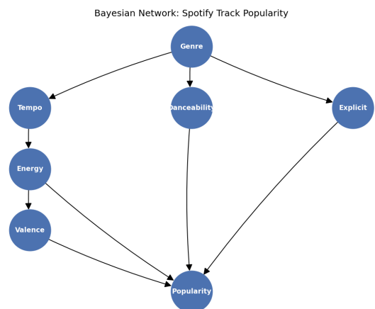
Figure 1: The custom Bayesian Network relating genre and audio features to track popularity.
