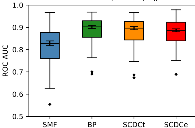
School network, T = 18 , \tau_w = 6h
