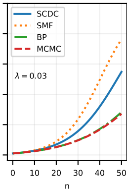
RRG ( k = 4 )
