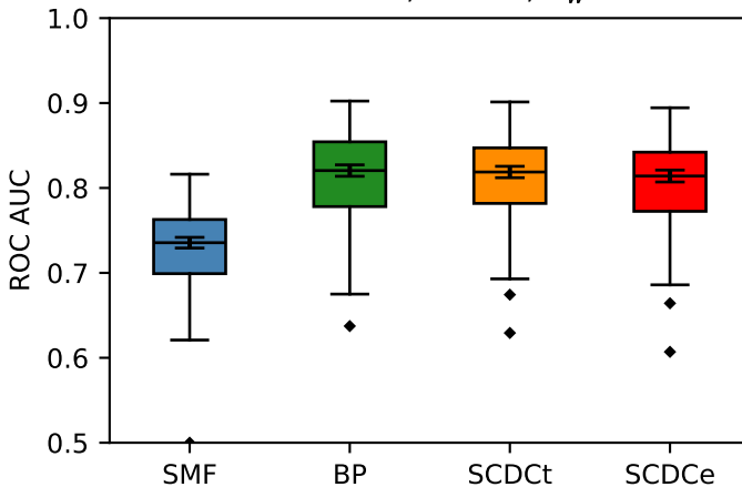
School network, T = 18 , \tau_w = 6h
