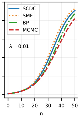
RRG ( k = 15 )
