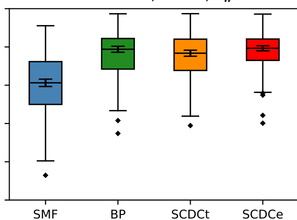
School network, T = 36 , \tau_w = 3h
