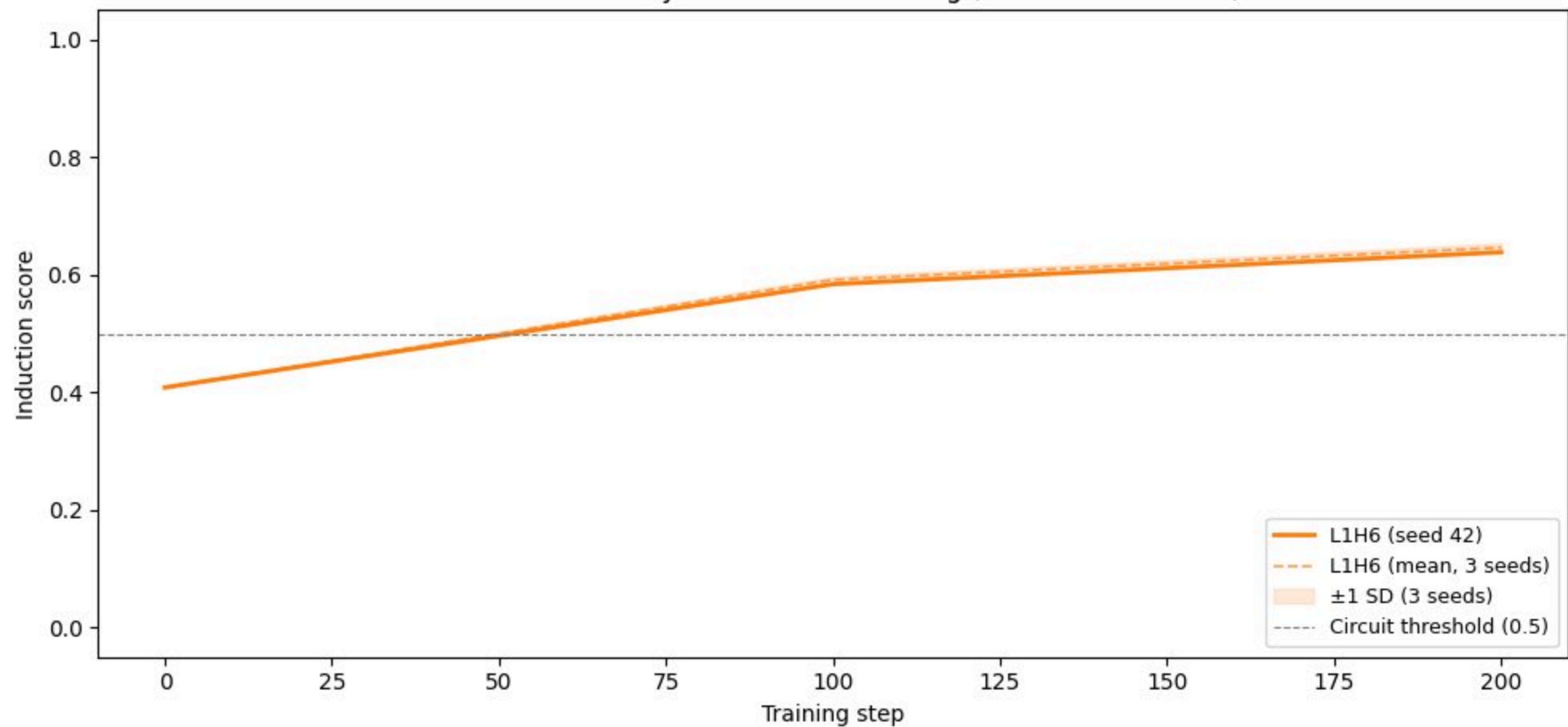
Induction score: Python code fine-tuning (3-seed mean \pm SD)
