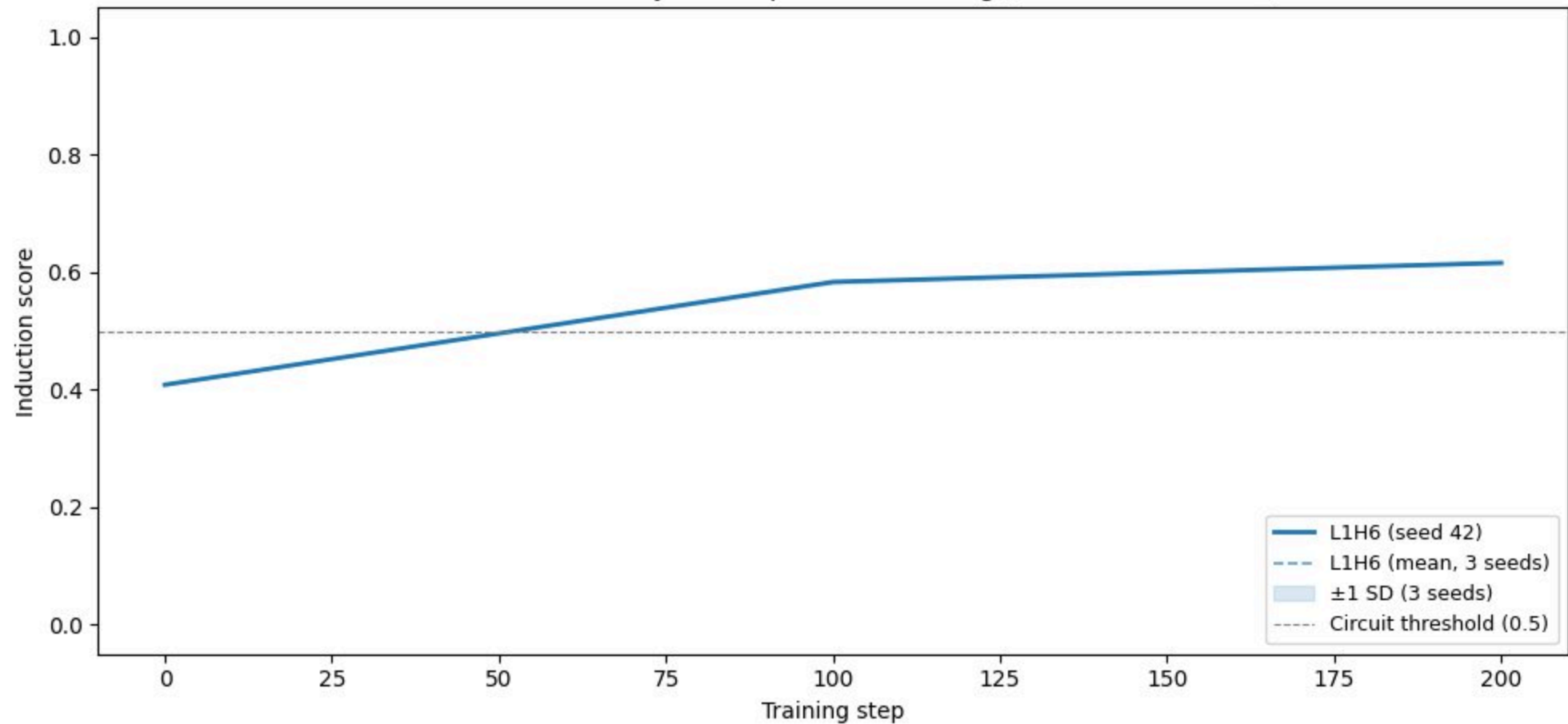
Induction score: TinyStories prose fine-tuning (3-seed mean \pm SD)
