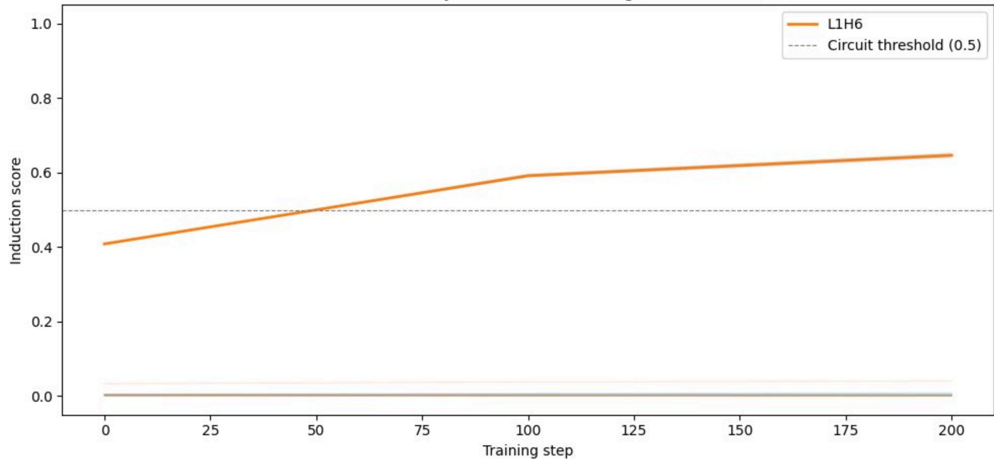
Induction score: Python code fine-tuning (Mean \pm 1 SD)
