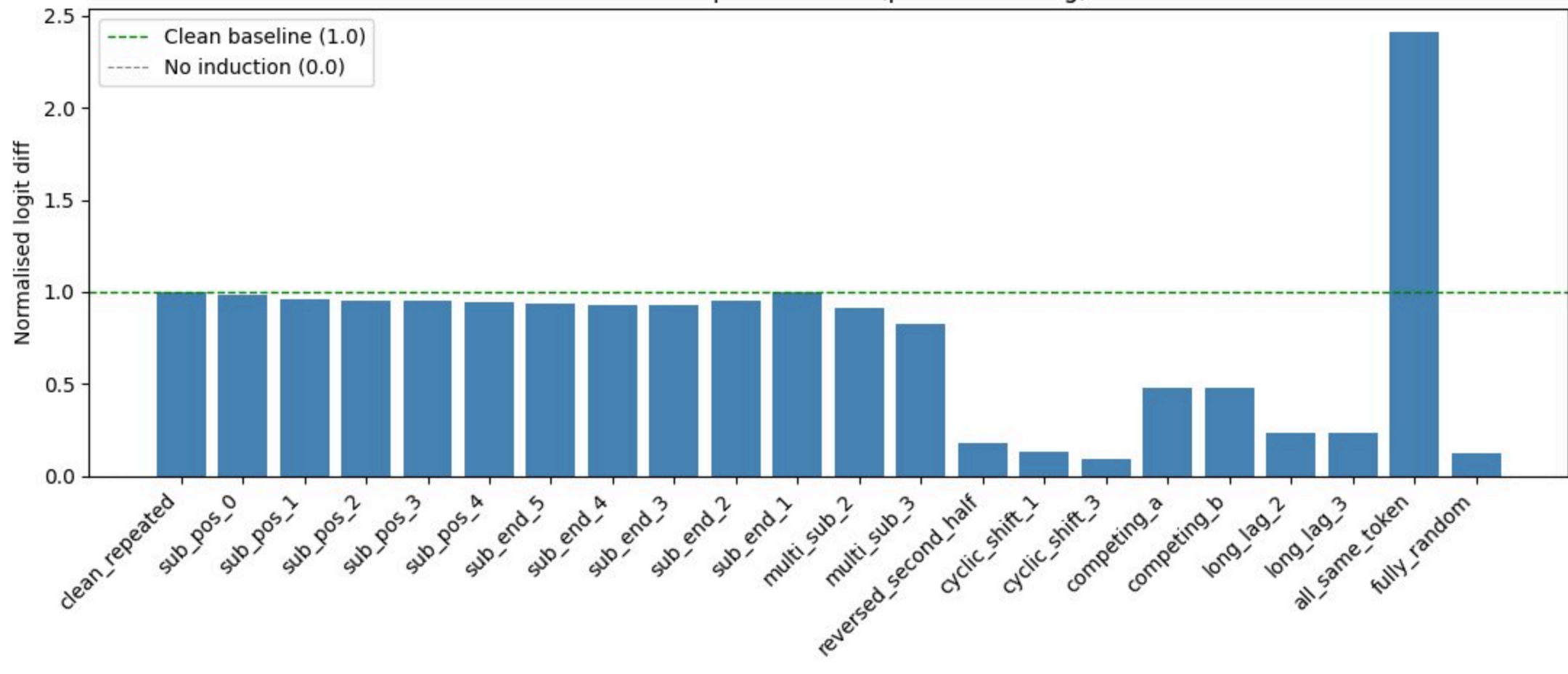
Adversarial probe results (post fine-tuning)
