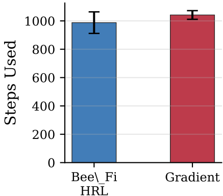
Episode Length
