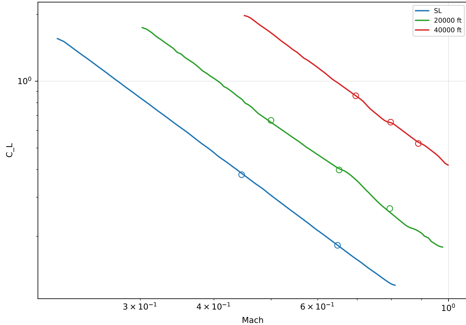
replotted from CSV (open circles = flight conditions)
