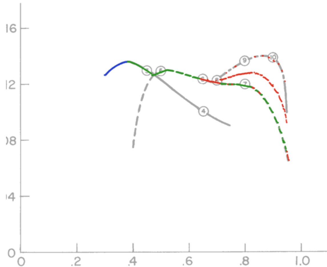
p.227 C_delta_a (rad^-1) — trace on scan
