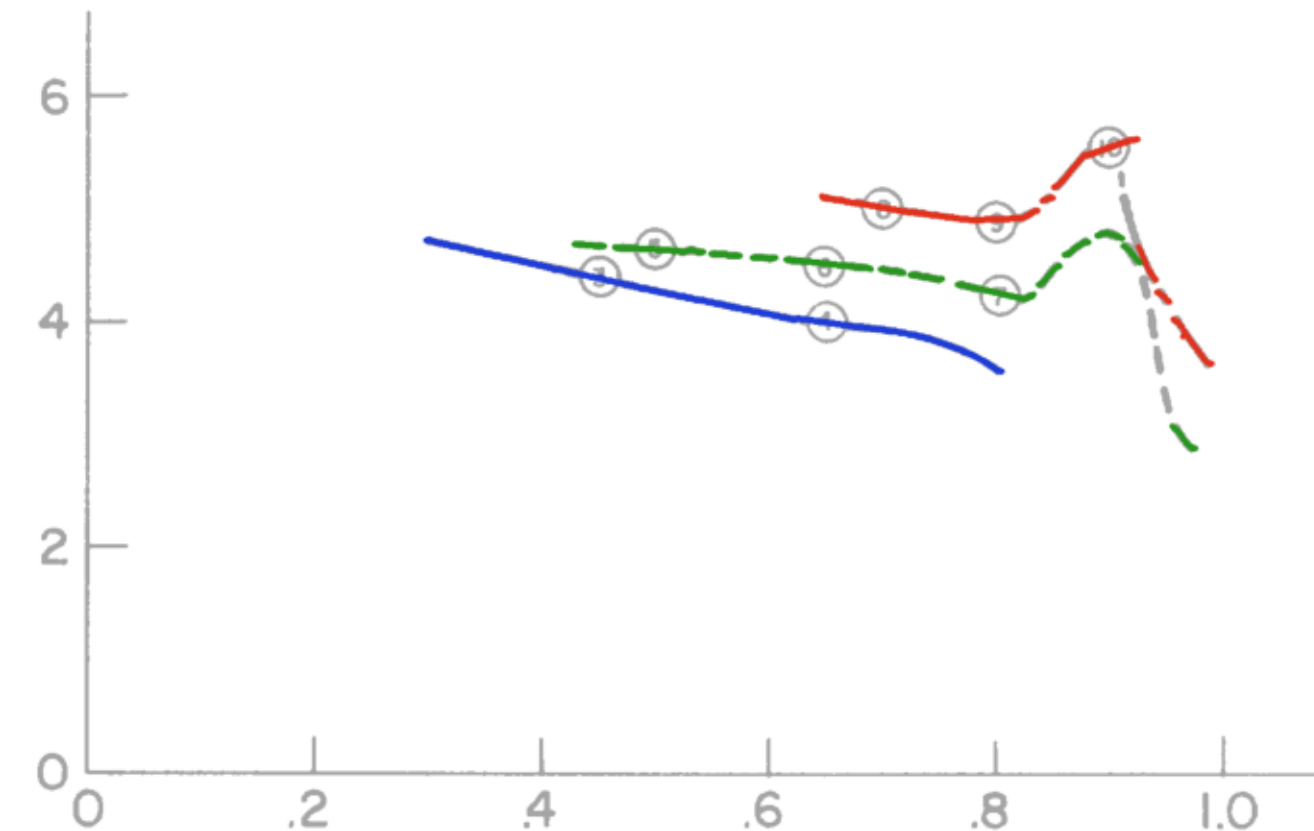
p.220 C_Lalpha (rad^-1) — trace on scan
