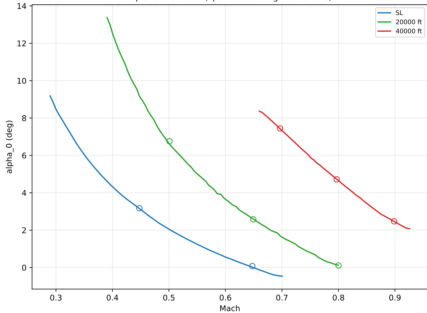
replotted from CSV (open circles = flight conditions)
