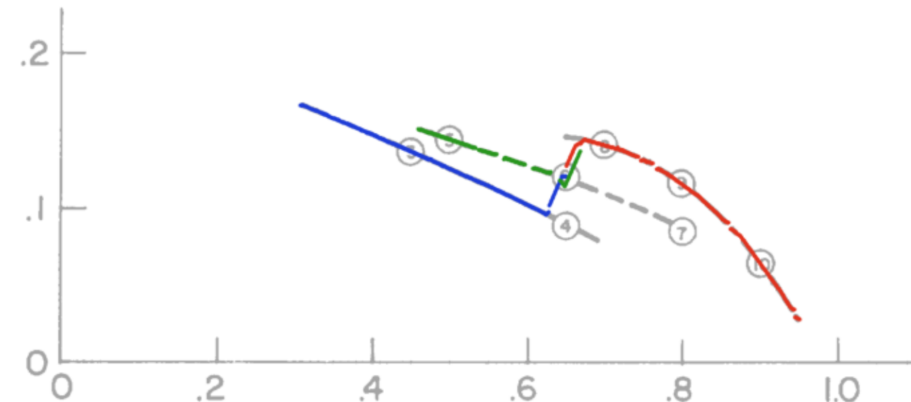
p.228 C_ydelta_r (rad^-1) — trace on scan
