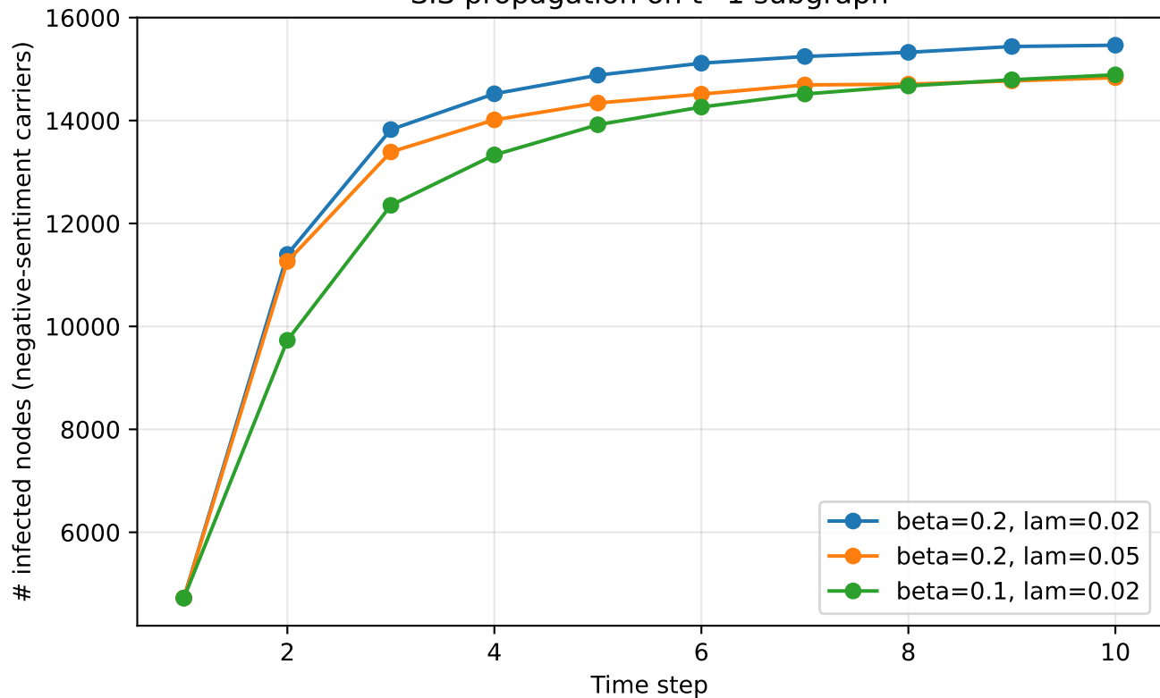
SIS propagation on t=1 subgraph
