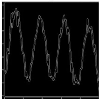
Canny: histogram_00174.png
