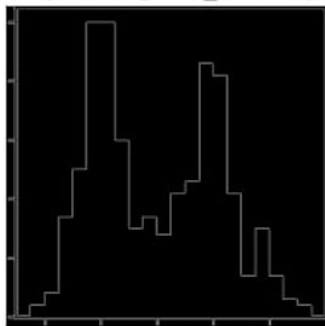
Canny: histogram_00174.png
