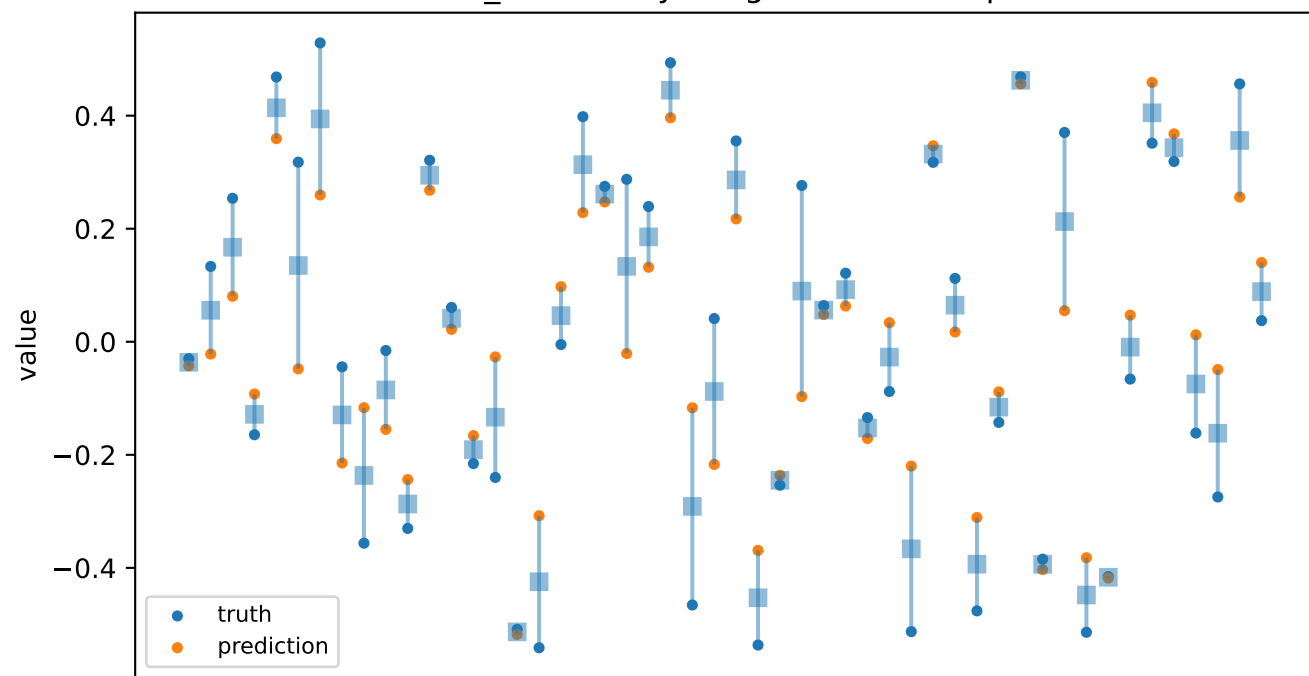
coef_4 - Primary astigmatism - oblique
