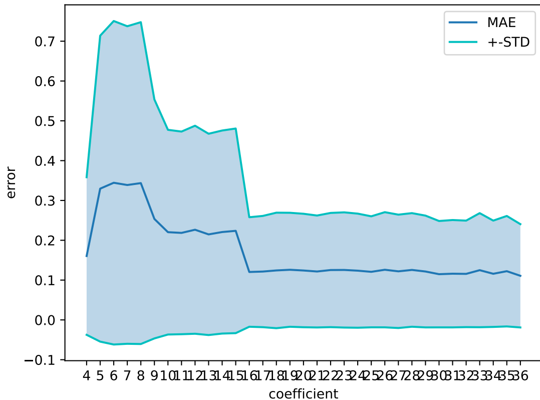
MAE with standard deviation for each coefficient
