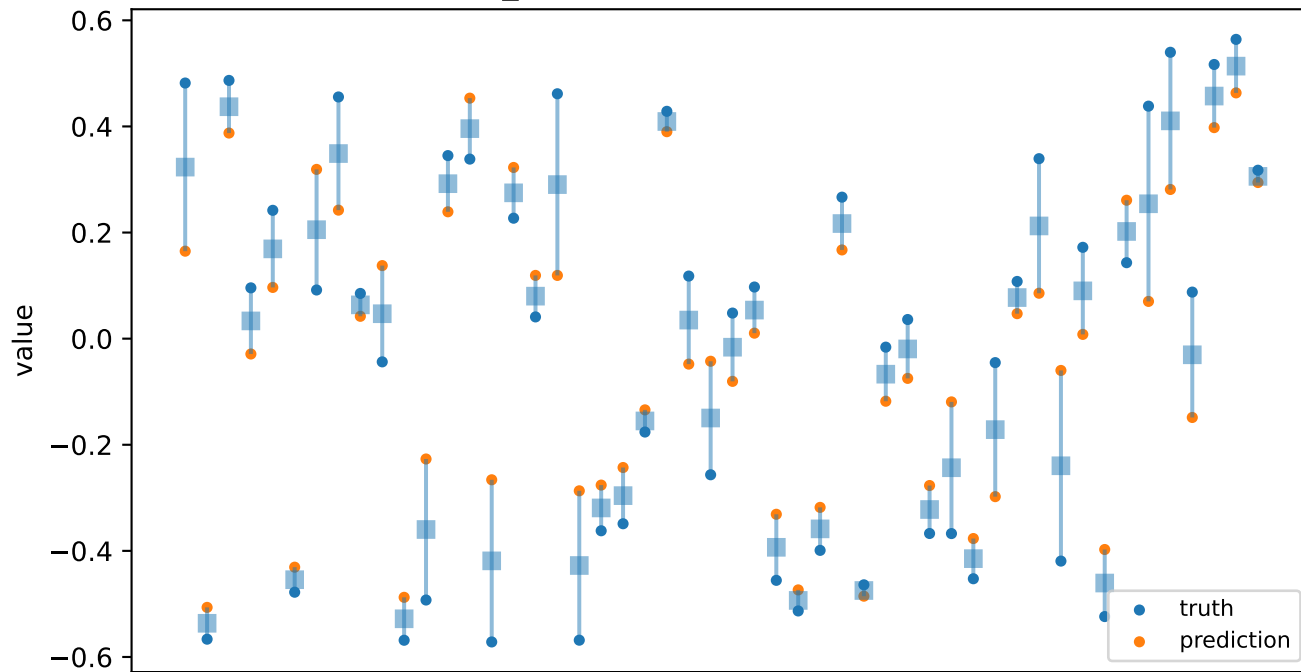
coef_5 - Primary astigmatism - vert.
