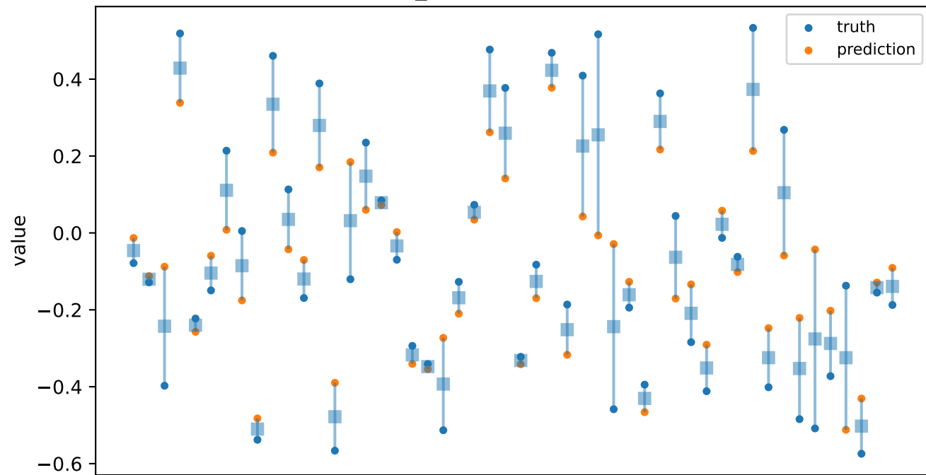
coef_6 - Primary coma - X
