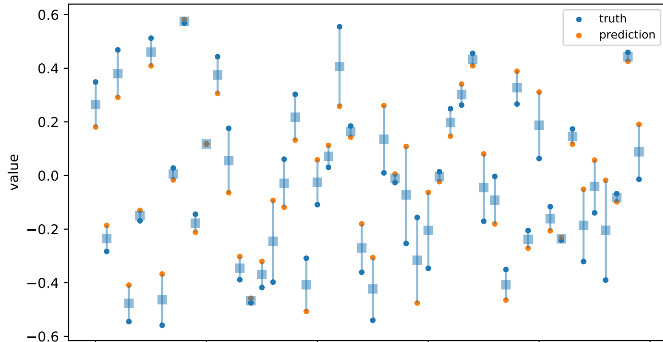
coef_8 - Primary spherical aberration
