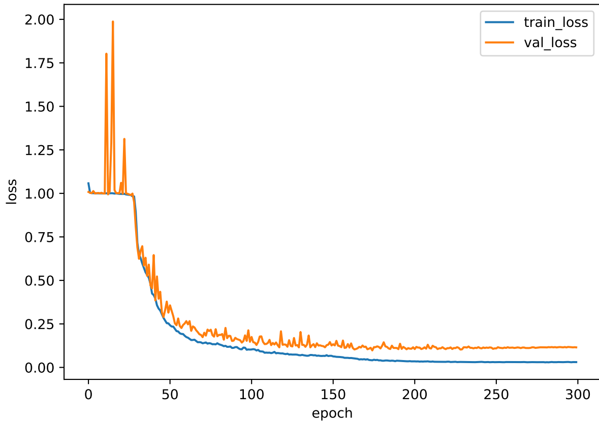
Training loss
