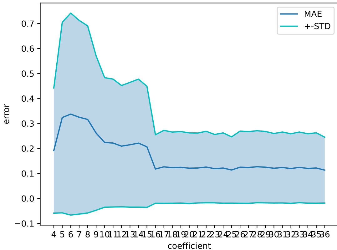
MAE with standard deviation for each coefficient
