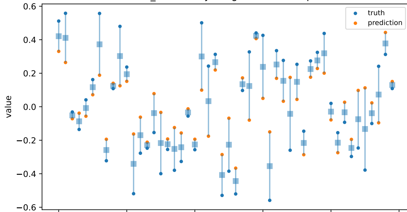
coef_6 - Primary coma - X
