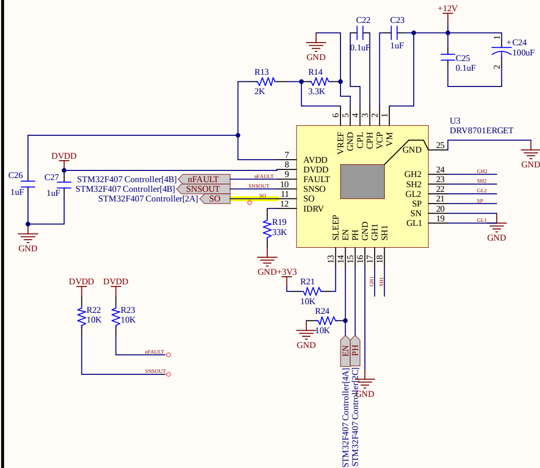
Motor Driver DRV8701
