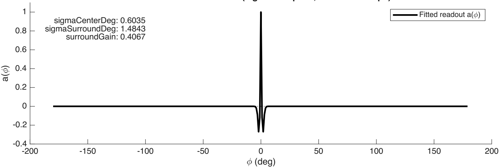
MT population responses to probes (signed template; flat readout)
