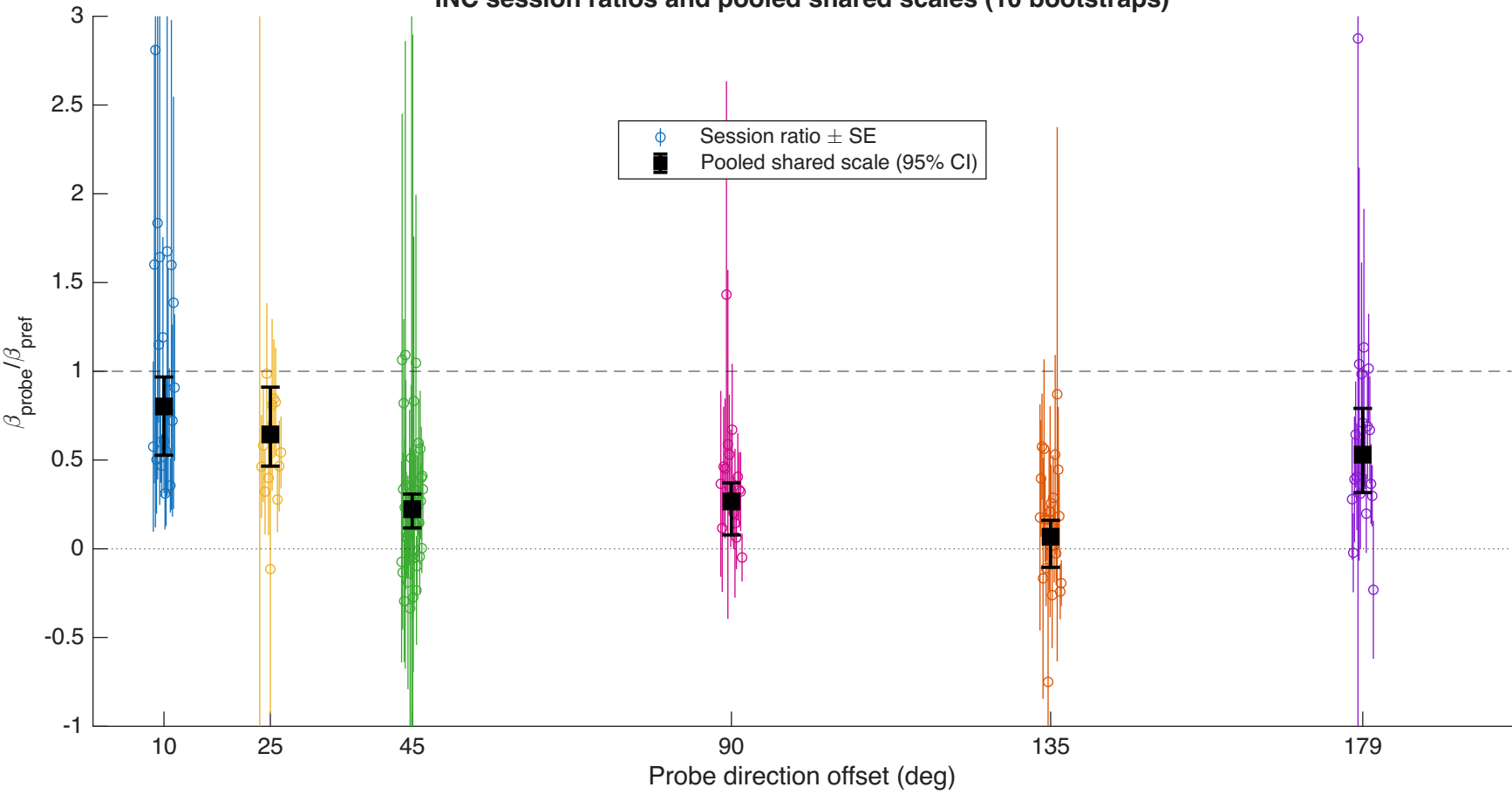
INC session ratios and pooled shared scales (10 bootstraps)
