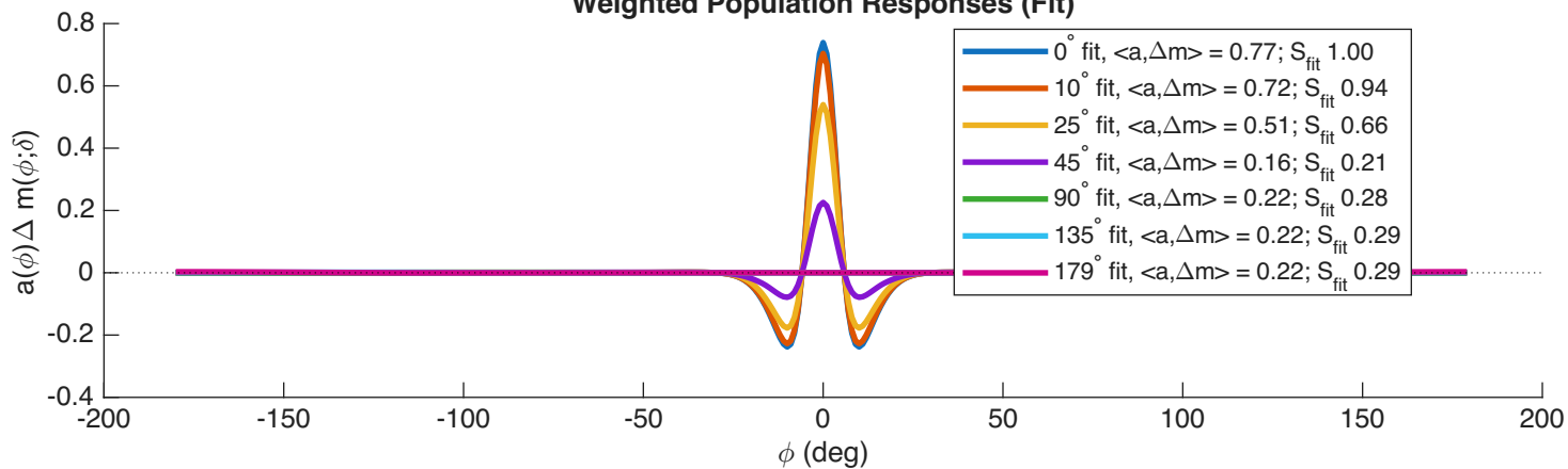
Weighted Population Responses (Fit)
