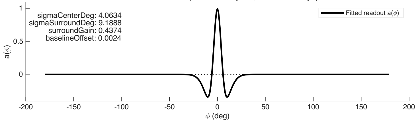
MT Population Responses to Probes (rectified template; Flat Readout)
