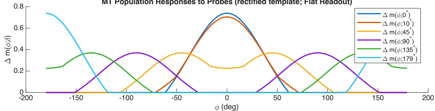
Weighted Population Responses (Fit)
