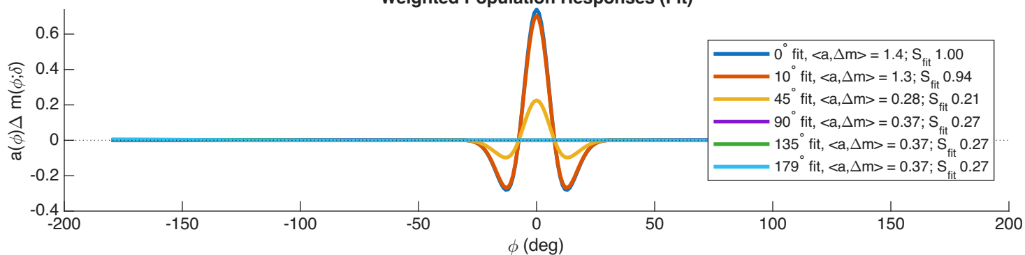
Weighted Population Responses (Fit)
