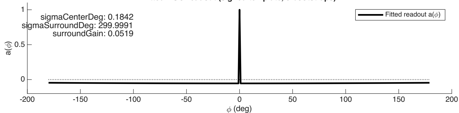
MT Population Responses to Probes (signed template; Flat Readout)
