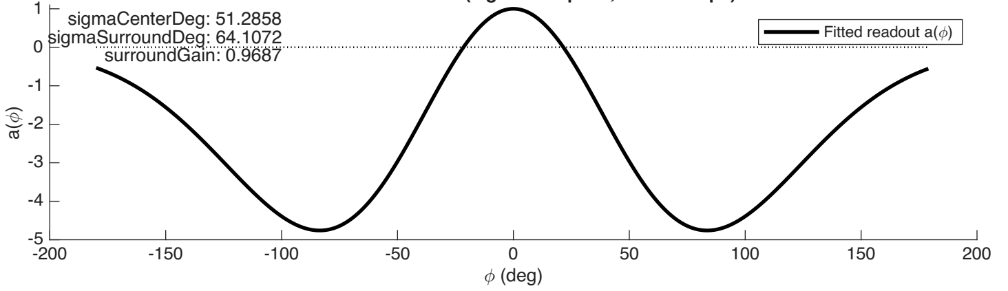
MT Population Responses to Probes (signed template; Flat Readout)
