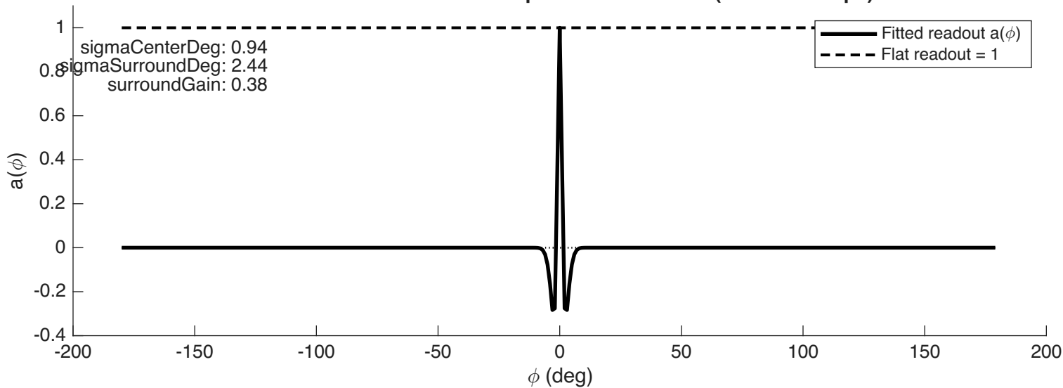
MT Population Responses to Probes (Flat Readout)
