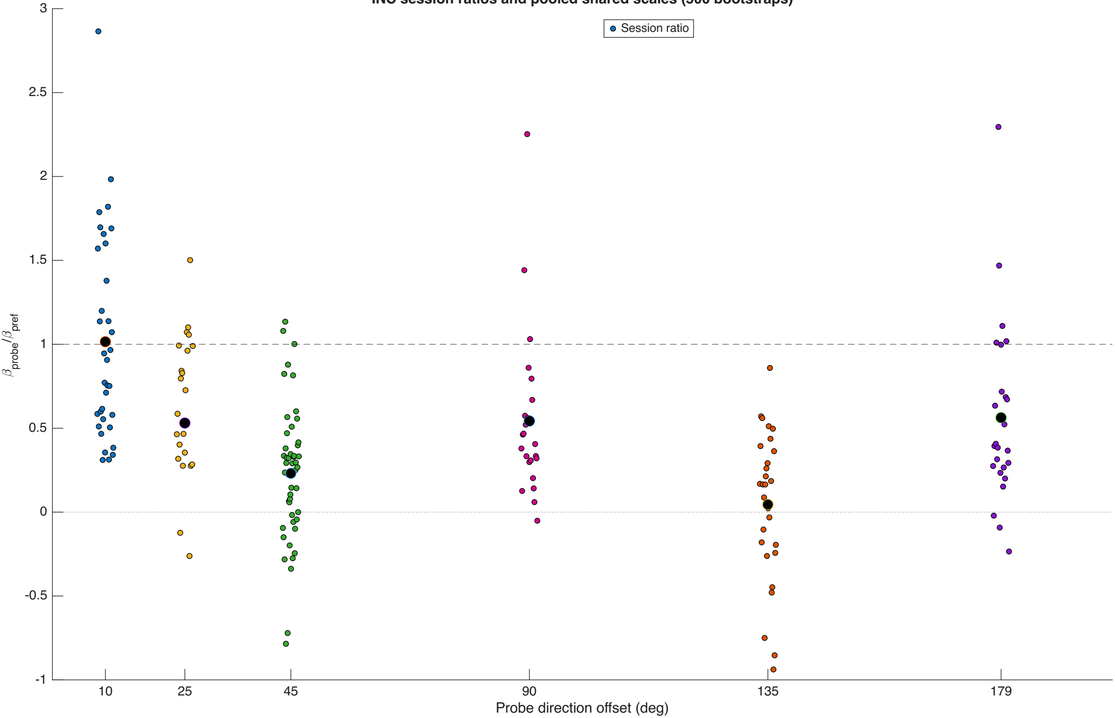
INC session ratios and pooled shared scales (500 bootstraps)
