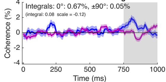
Coherence Decrements: No Change RDK Kernels
