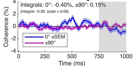
Coherence Decrements: Right RDK Kernels
