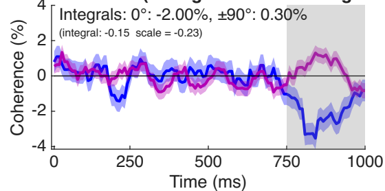
Coherence Decrements: Change RDK Kernels
