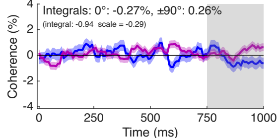
Coherence Decrements: Left RDK Kernels
