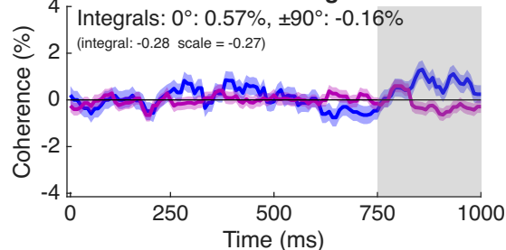
Coherence Increments: Right RDK Kernels
