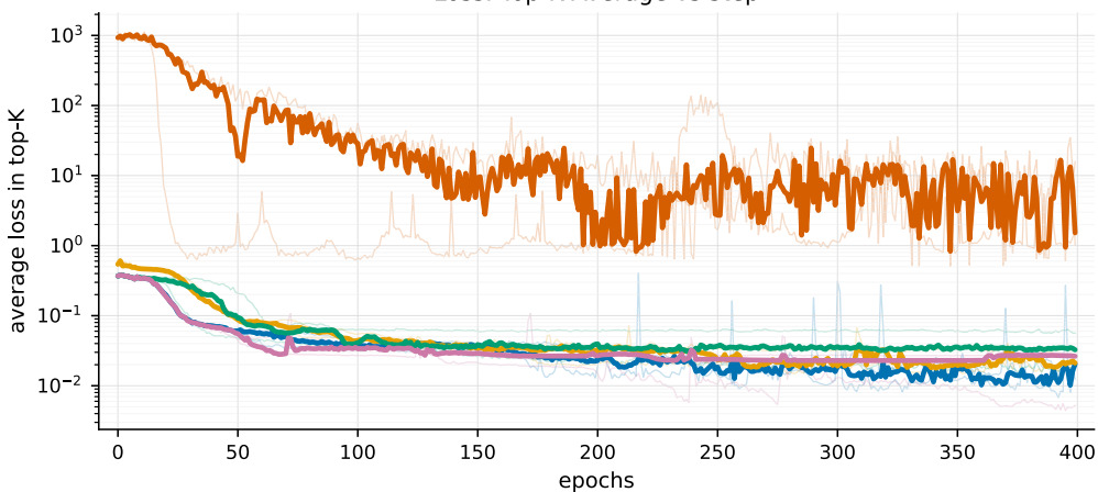
Loss: Top-K Average vs step
