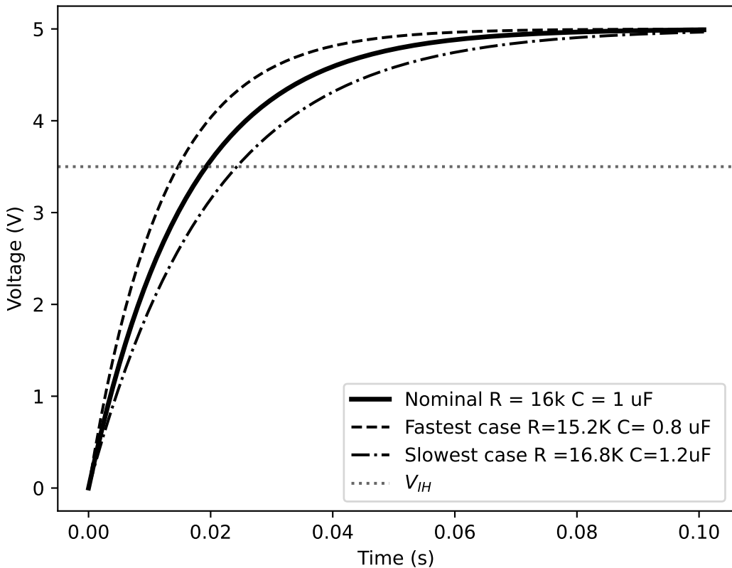
Capacitor charging for component tolerances
