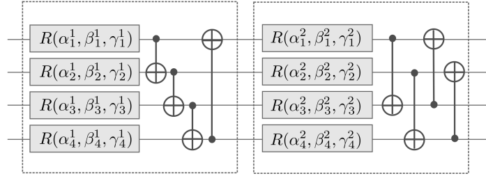
Figure 3.1: Example of two 4-qubit strongly entangling layers (ranges r = 1 and r = 2 , respectively) with rotations R and CNOTs as imprimitives, adapted from PennyLane (2026).
