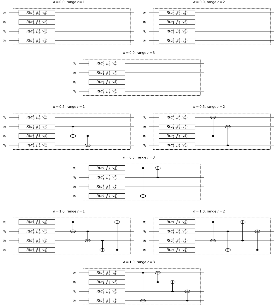
Figure 3.2: Example of the controlled CCC ansatz for M = 4 qubits and three interaction ranges r = 1, 2, 3 . Each panel shows one layer consisting of local rotations R(\alpha_i^\ell, \beta_i^\ell, \gamma_i^\ell) , followed by the active CNOT couplings selected by the entanglement-control parameter.
