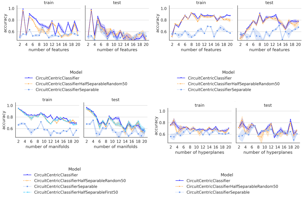
Figure 3.4: Train and test accuracy curves for the completed geometric benchmark families: linearly separable, hidden manifold, hidden manifold diff and hyperplanes diff.
