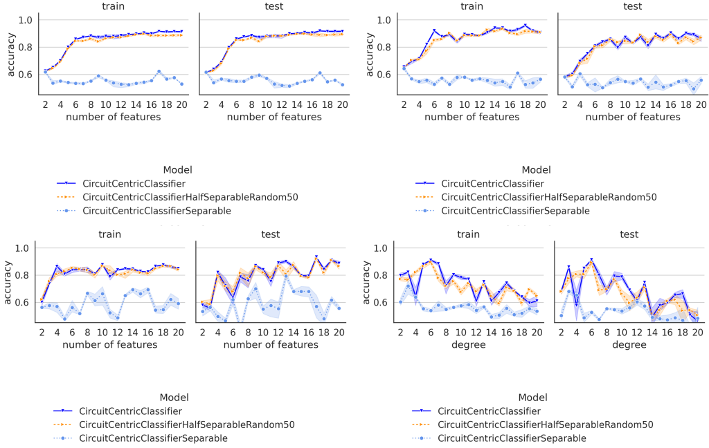
Figure 3.5: Train and test accuracy curves for MNIST PCA, MNIST PCA small, two curves, and two curves diff
