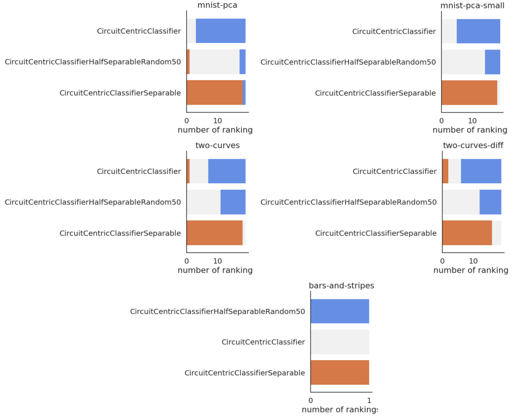
Figure 3.3: Per-family ranking plots for MNIST PCA, MNIST PCA small, two curves, two curves diff, and bars and stripes.
