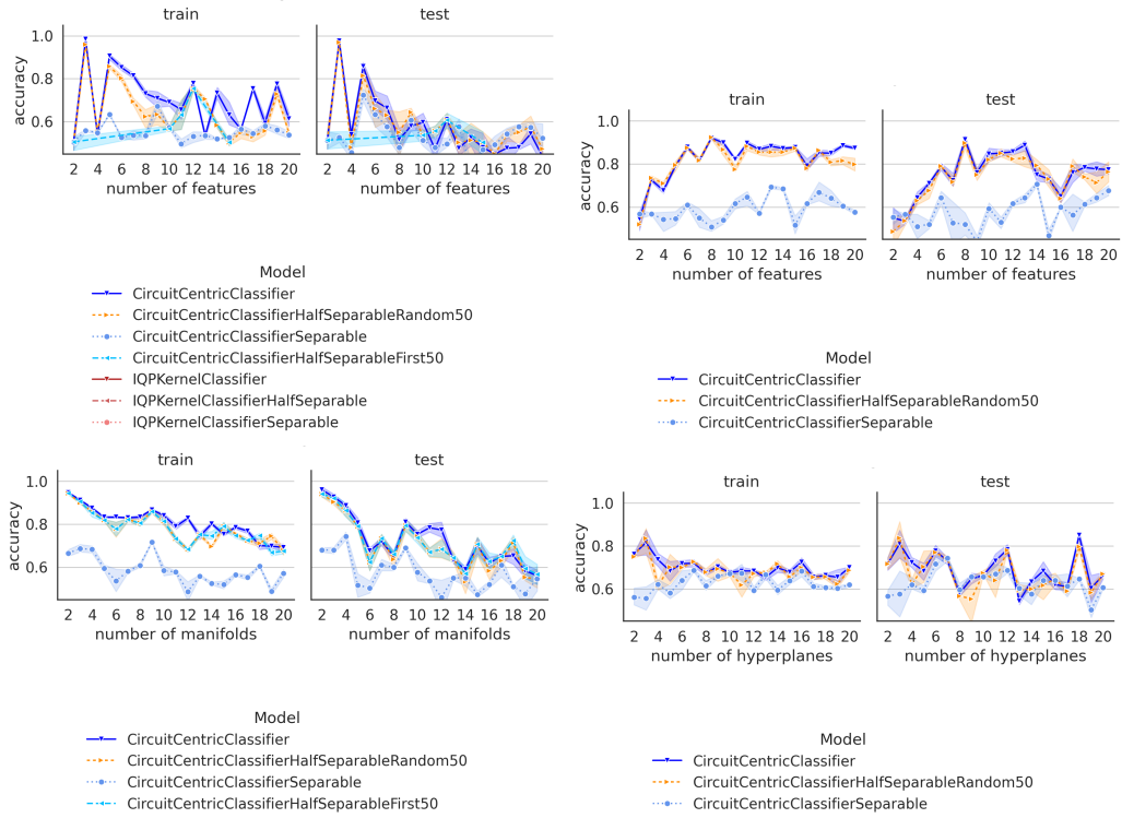
Figure 3.4: Train and test accuracy curves for the completed geometric benchmark families.
