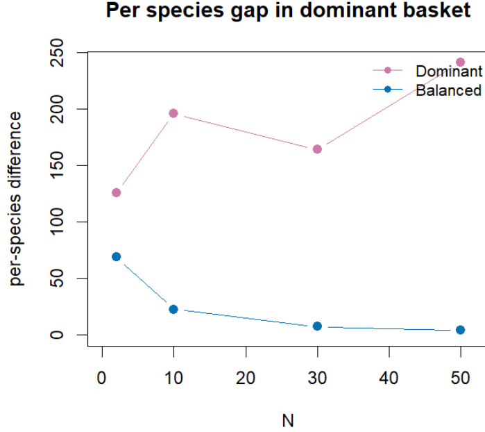
Figure 4: Robustness with one persistently dominant species. Per-species welfare does not vanish when one species’ participation dominates, even as basket size increases, relative to a balanced basket.
