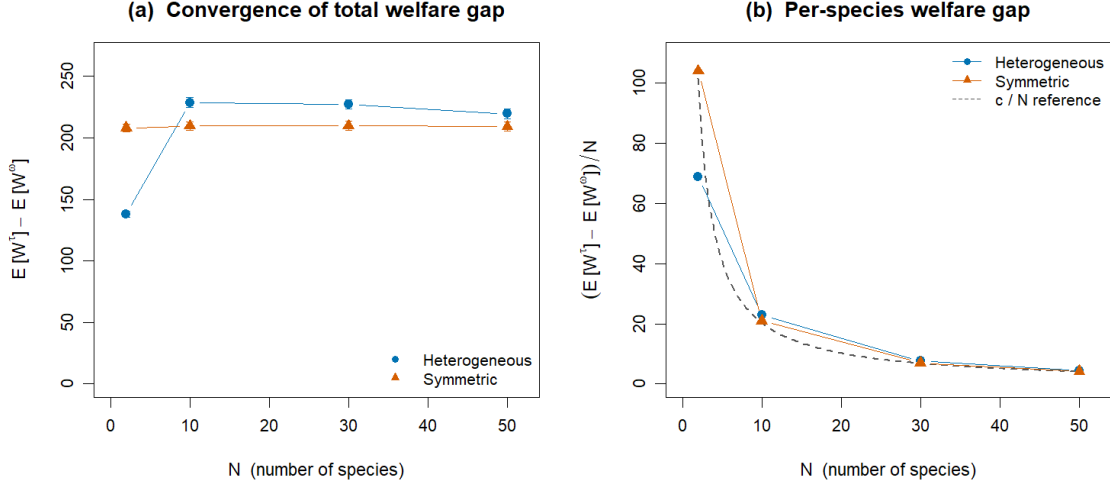
Figure 2: Left: expected total welfare difference \mathbb{E}[\mathcal{W}^\tau] - \mathbb{E}[\mathcal{W}^\omega] per basket size N , the difference converges to a positive constant. Right: the per-species difference vanishes at rate O(1/N) .
