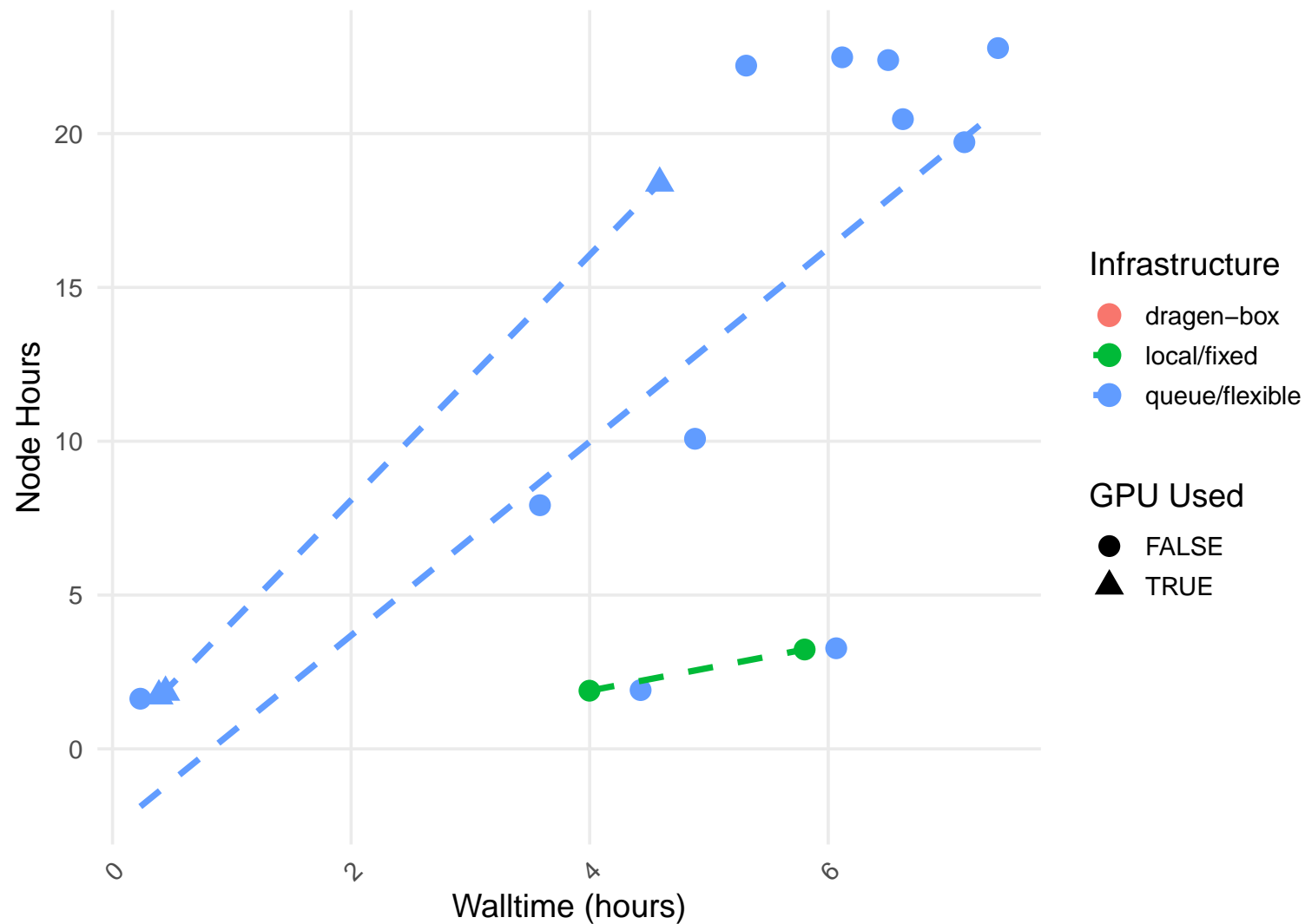
Node Hours vs Walltime
