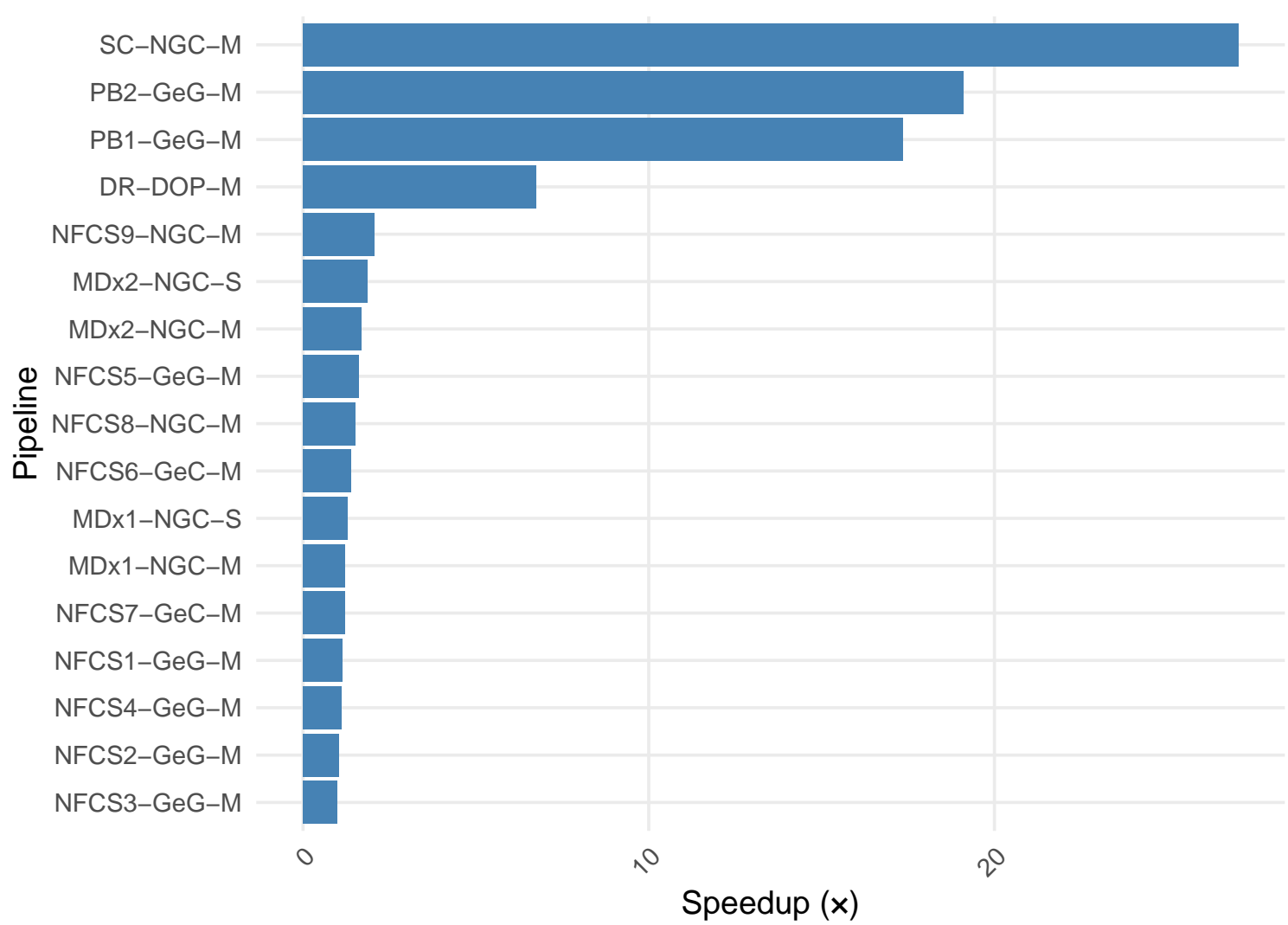
Speedup Relative to Slowest Pipeline
