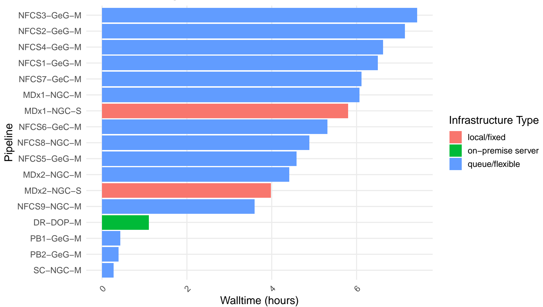
Walltime Comparison
