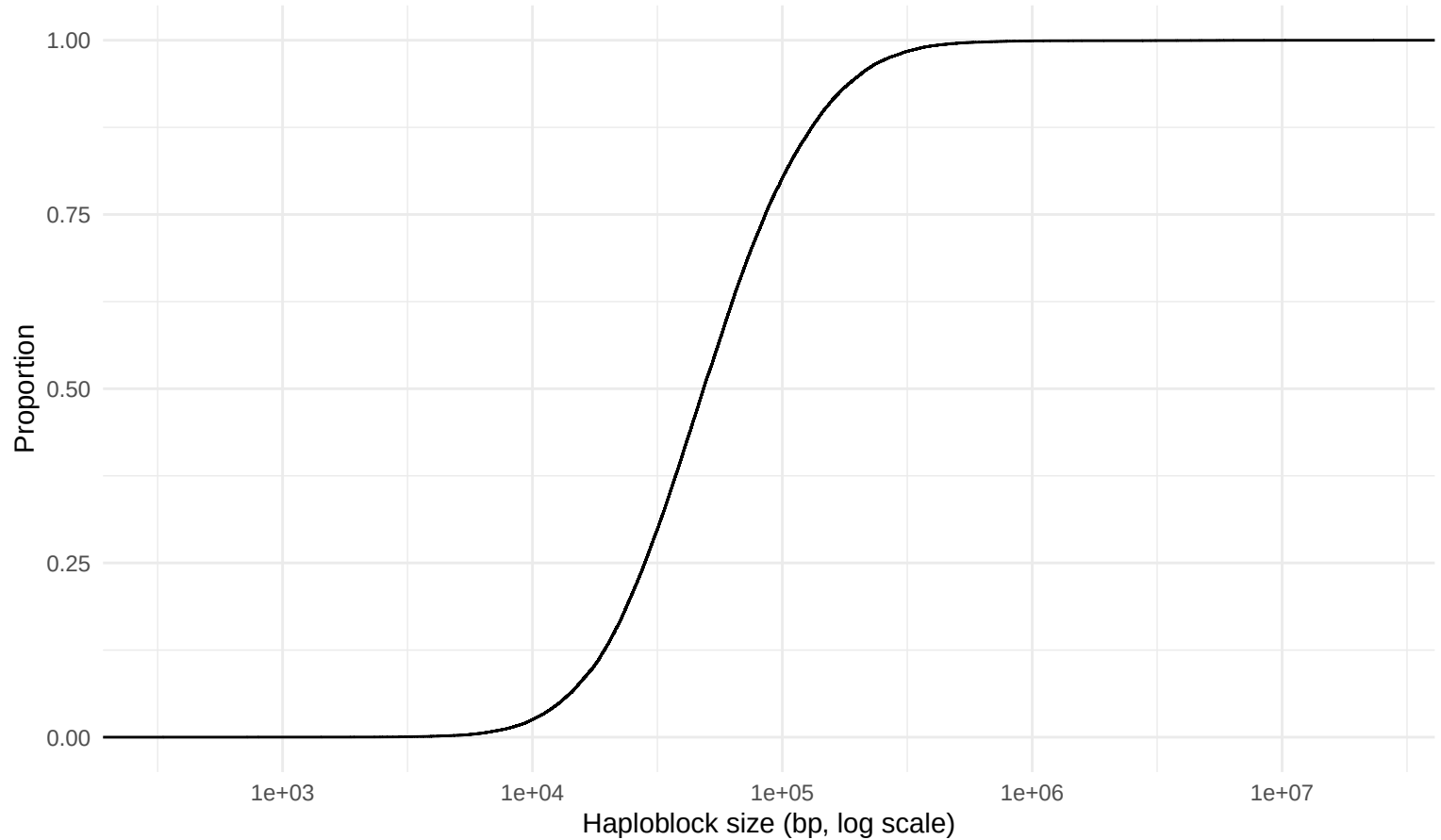
Cumulative Distribution of Haploblock Sizes
