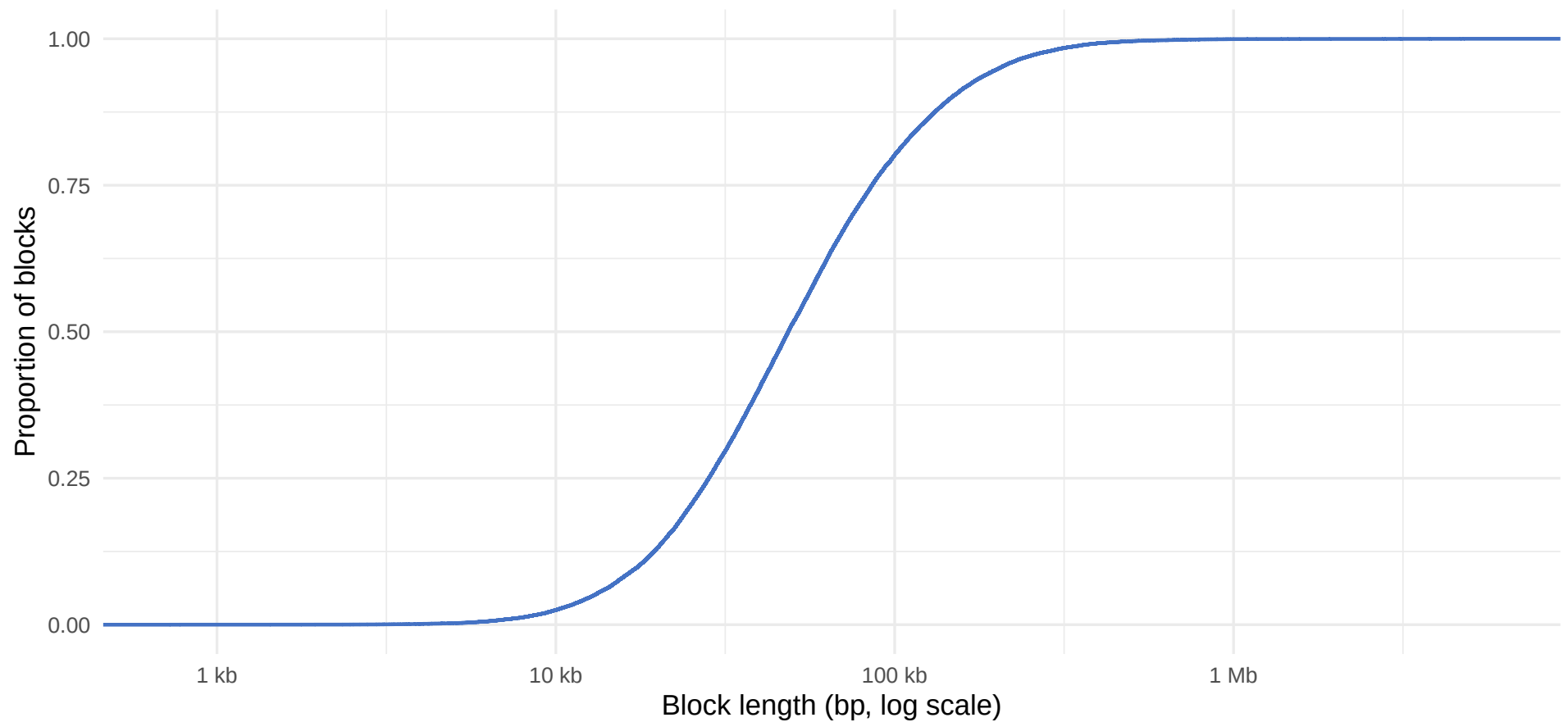
Cumulative distribution of haploblock sizes
