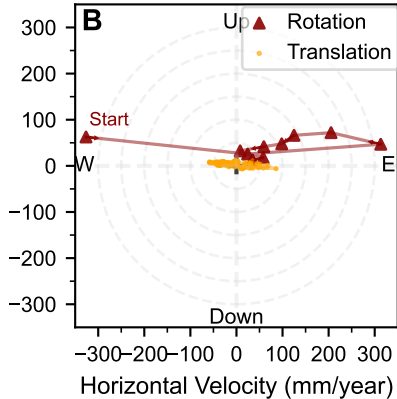
Roto-Translational Phase
