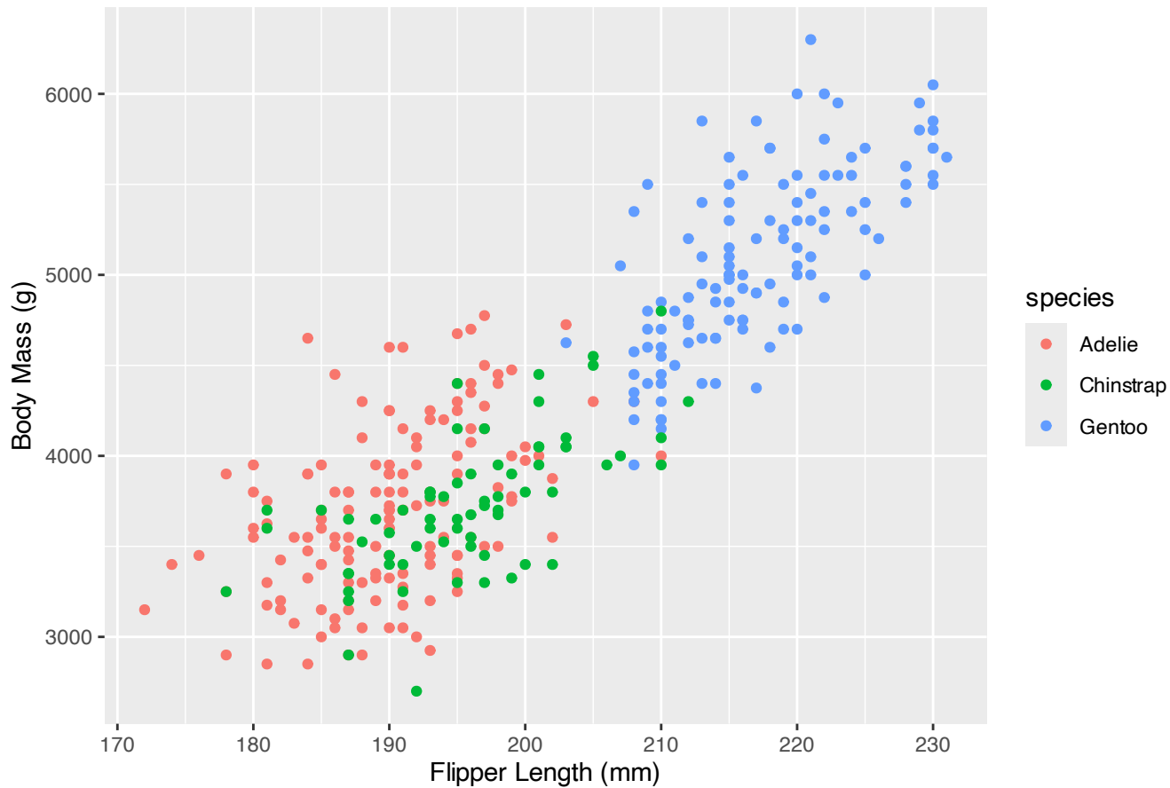
Flipper Length vs Body Mass
